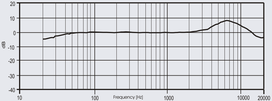
Frequency Response
